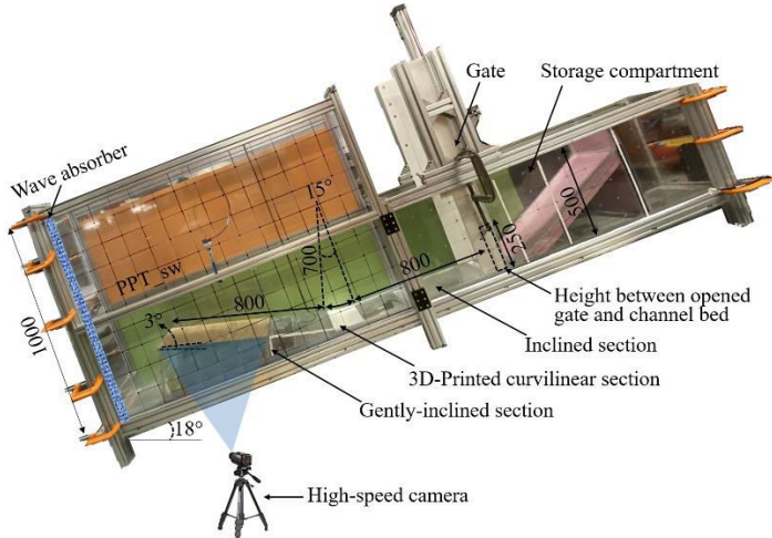
Figure 3. Side view of the flume for studying submarine debris flows
